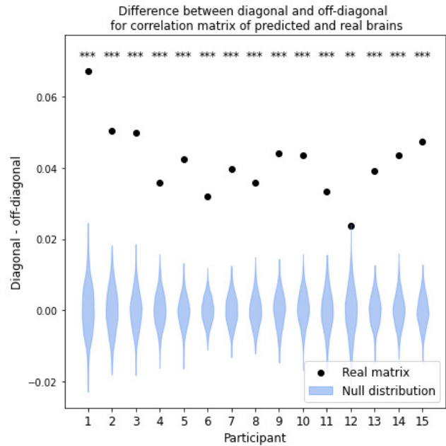
Figure 2. Per-participant fMRI prediction permutation analysis.
